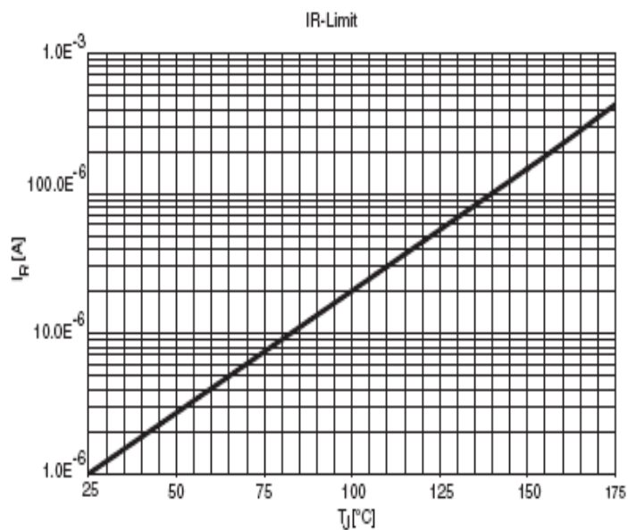
Figure 4. Maximum Reverse Current
