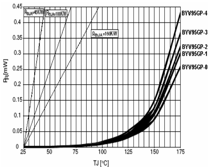
Figure 3. Maximum Reverse Power Dissipation
